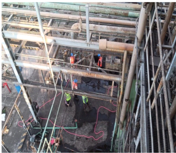
250mm RCC Slab Breaking in progress
